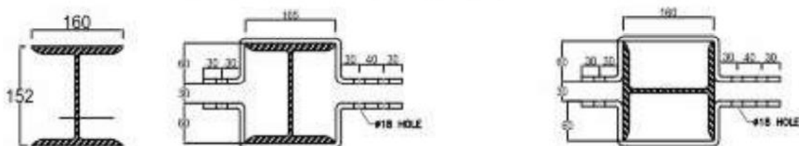
STAY SET CLAMP ( TYPE A )
